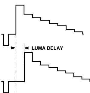
Figure 29. Luma Delay
