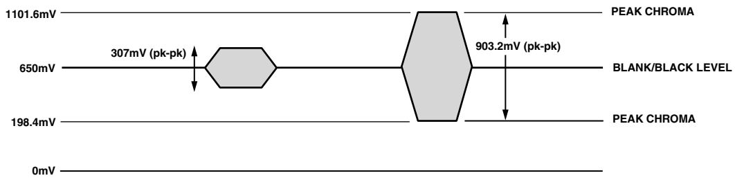
Figure 114. NTSC Chroma Video Levels
