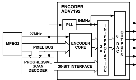
Figure 34. Block Diagram Using the ADV7192 in Progressive Scan Mode
